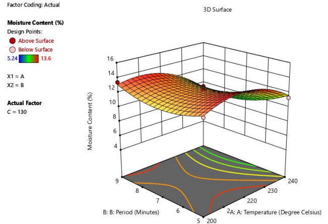
Fig 3. 3D surface for the effect of baking temperature and baking period on the moisture content
